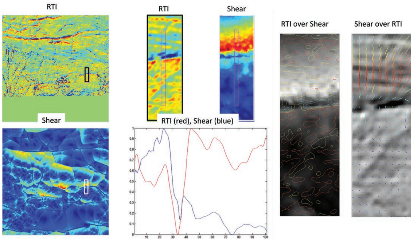
FIGURE 10. Map of RTI-generated slope magnitudes (top left) and the corresponding absolute of the gradient of displacement (strain) map (bottom left), where red indicates large negative or positive strain and blue indicates low strain. The top middle panel shows details of areas outlined in the corresponding maps. Within each detail is a smaller outline of the data plotted in the graph below. The data sets in the graph are normalized to facilitate comparison. On the right are overlays; “RTI over Shear” shows color-coded surface slope data overlaid onto a grayscale map of the shearography data, whereas “Shear over RTI” shows the color-coded strain vectors overlaid onto an RTI-generated image of the slope of the topology, where white and black indicate large positive or negative surface slope and gray indicates nearly no surface slope.
